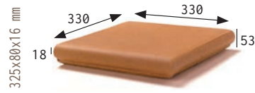
ESQUINA REDONDEADA ROUNDED STAIR-TREAD CORNER
